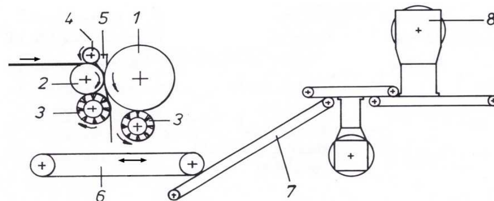
Buffing Line "Fulminosa+ De-dusting Machine 661 B" + dust removal + storing filter + compacting system + stacker
